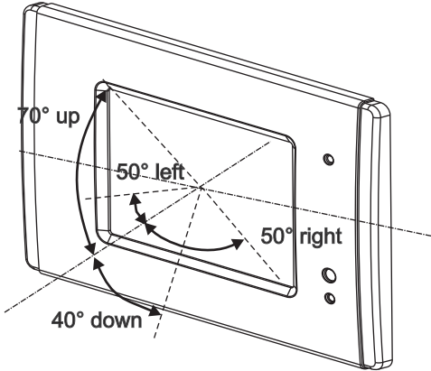
Figure 3. Wall Mounted touchscreen unit's viewing angles
