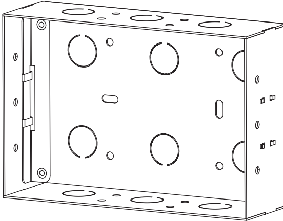
Figure 7. The wall box for use with stud/plasterboard walls.
