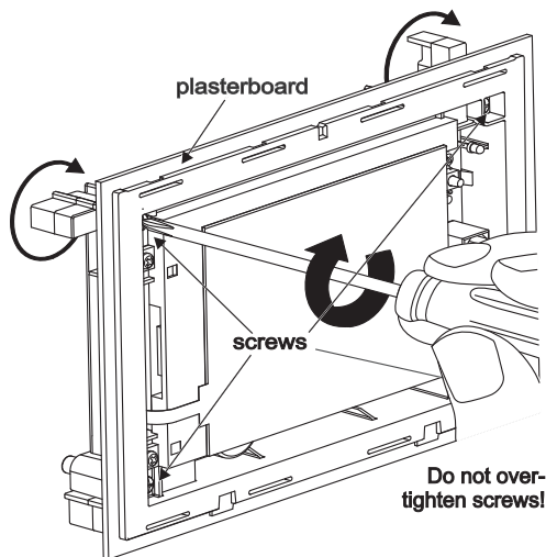
Figure 6. Tighten the screws and the mounting flaps rotate and clamp the wall
