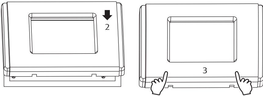
Figure 10. Attaching the fascia (Wall Mounted Touchscreen)
