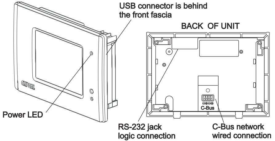
Figure 1. Wall Mount touchscreen connection points
