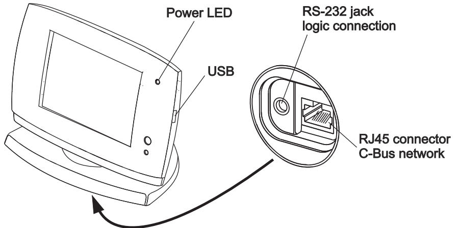
Figure 2. Desktop Touchscreen connection points
