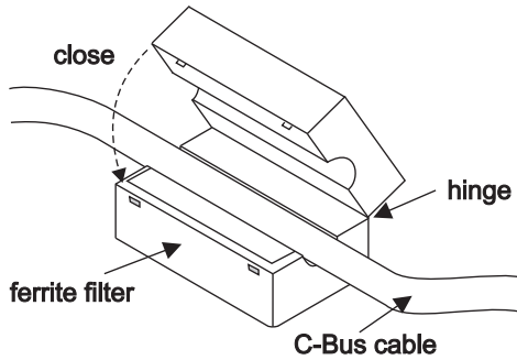
Figure 12. Ferrite filter placement on the C-Bus network cable
