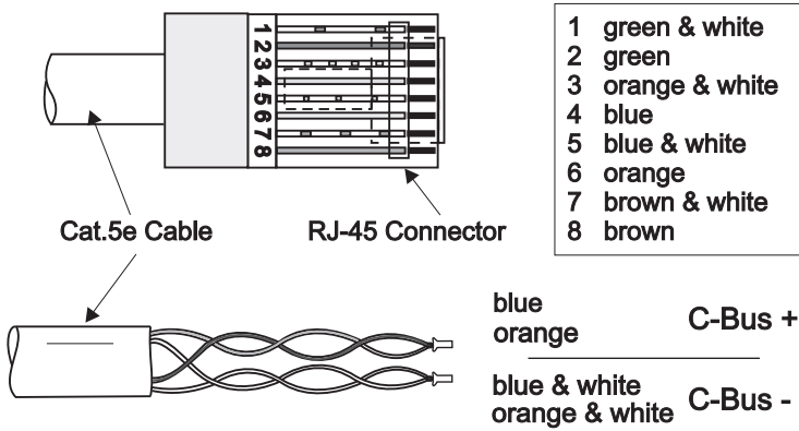
Figure 11. C-Bus network cable connections
