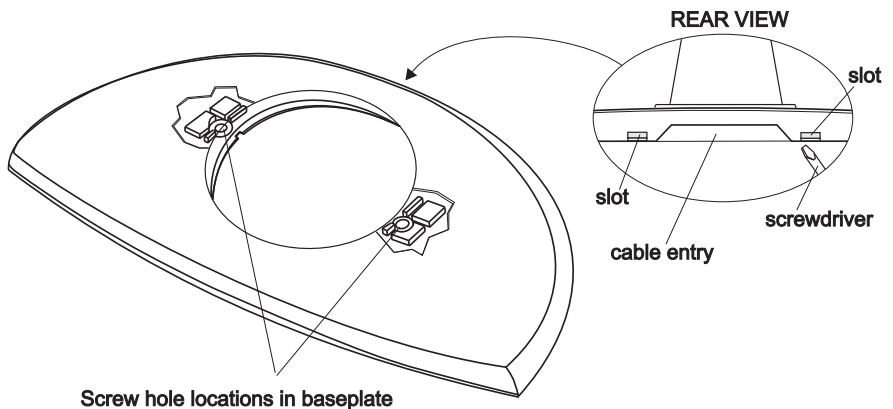
Figure 9. Mounting the Desktop Touchscreen
